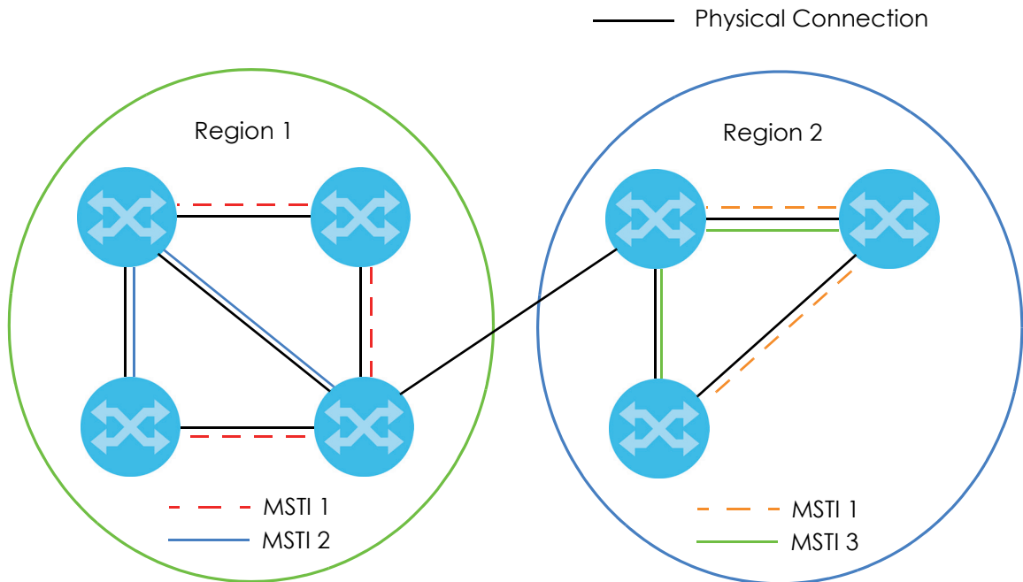
Figure 105 MSTIs in Different Regions
