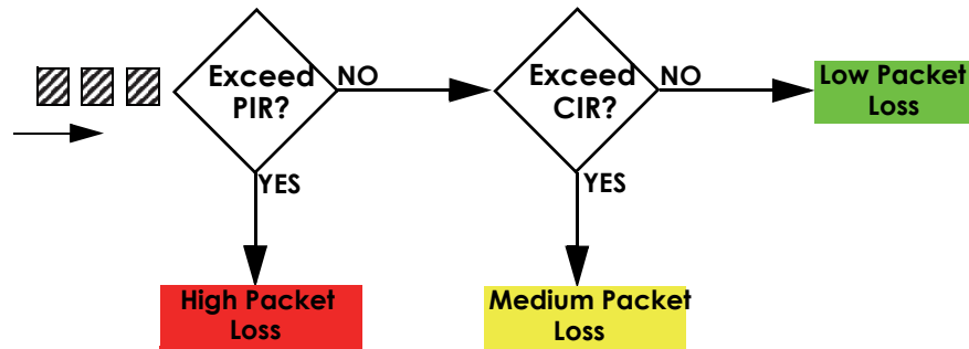
Figure 223 TRTCM-Color-blind Mode
