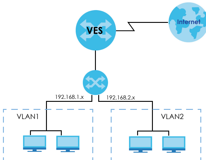
Figure 26 Initial Setup Example: Management IP Address
