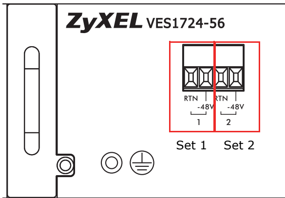
Figure 13 VES1724-56 DC Power Terminals
