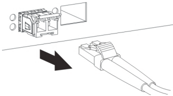
Figure 17 Opening the Transceiver's Latch Example
