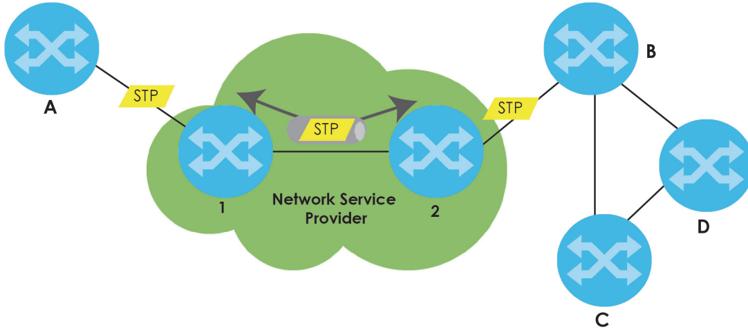
Figure 184 L2PT Network Example
