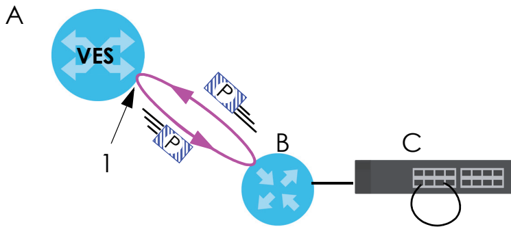
Figure 174 Loop Guard - Network Loop
