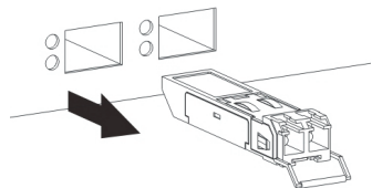
Figure 18 Transceiver Removal Example
