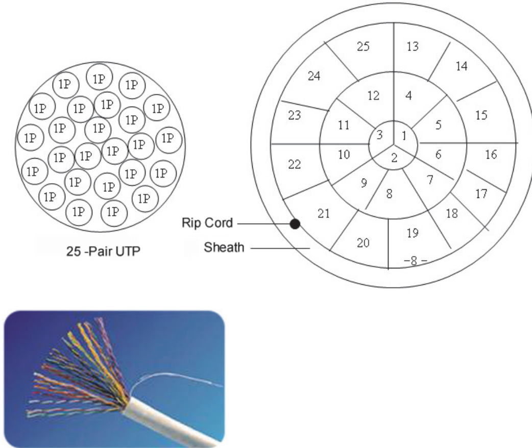
Figure 290 Telco-50 Cable Structure
