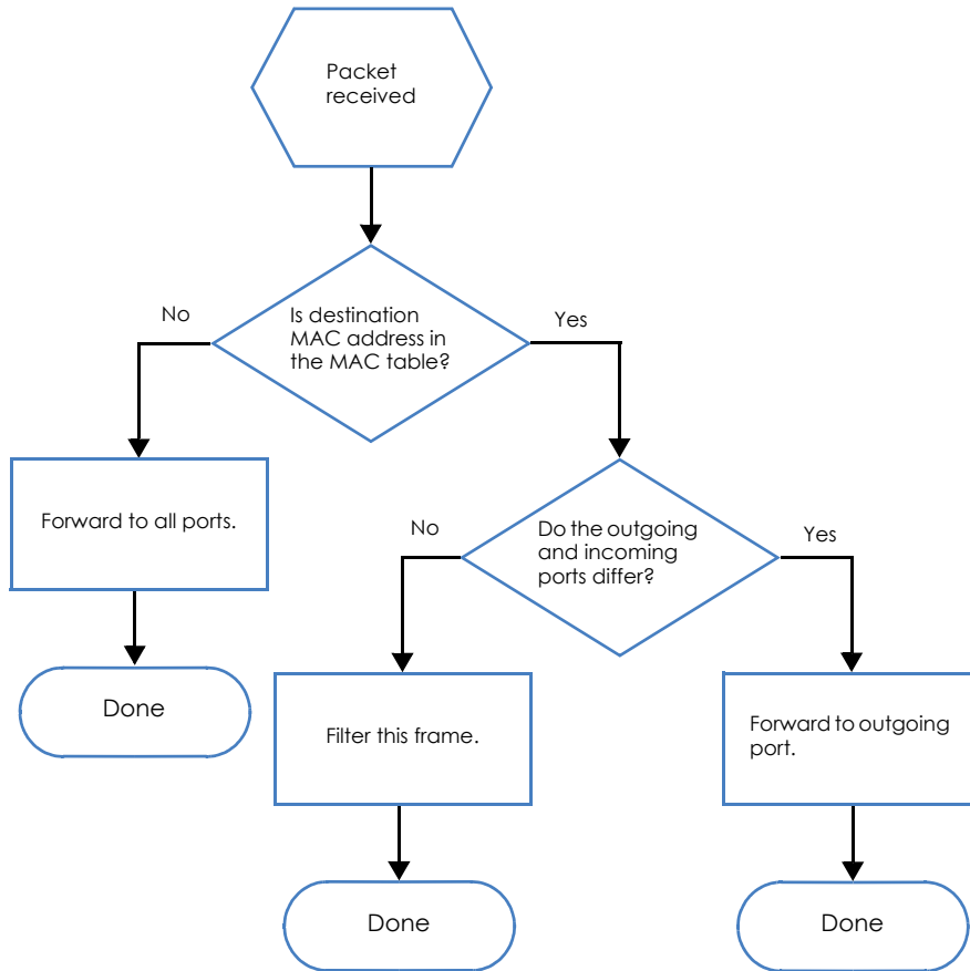
Figure 270 MAC Table Flowchart
