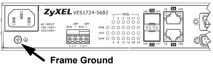
Figure 8 VES1724-56B2 Frame Ground
