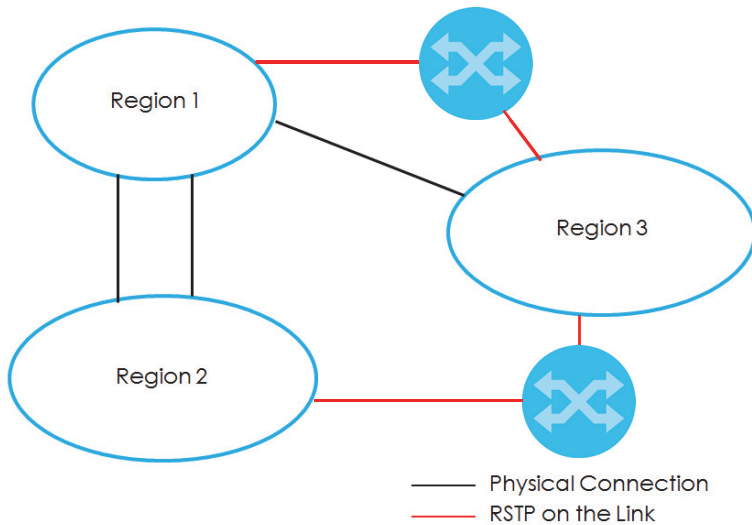
Figure 106 MSTP and Legacy RSTP Network Example
