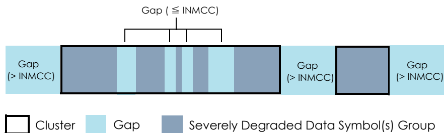
Figure 73 INM Cluster Example
