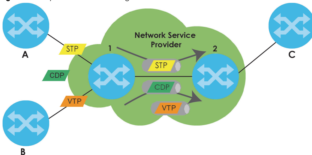
Figure 183 Layer 2 Protocol Tunneling Network Scenario
