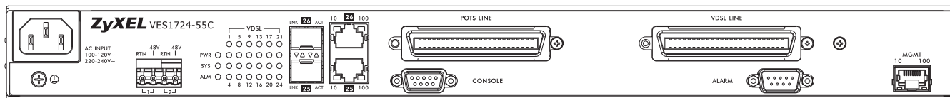
Figure 10 VES1724-56 Front Panel
