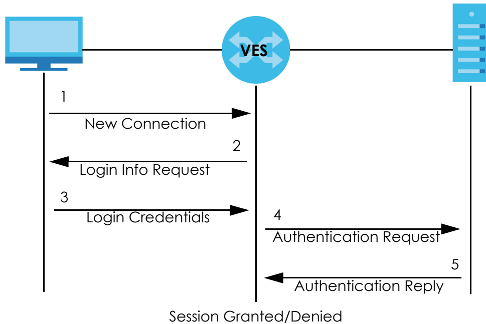
Figure 122 IEEE 802.1x Authentication Process
