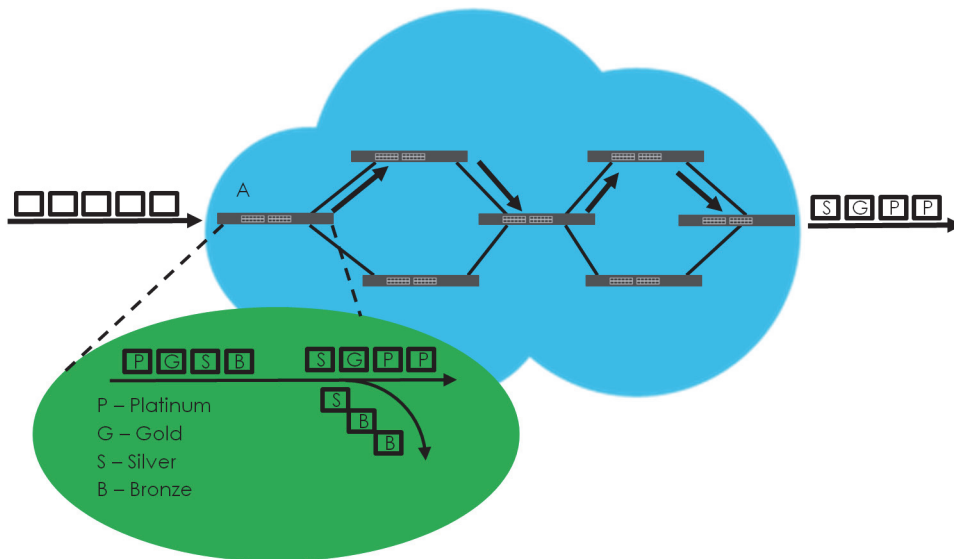
Figure 222 DiffServ Network
