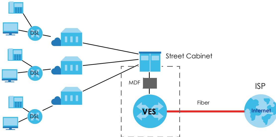
Figure 2 Curbside Application
