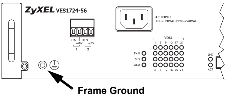
Figure 7 VES1724-56 Frame Ground
