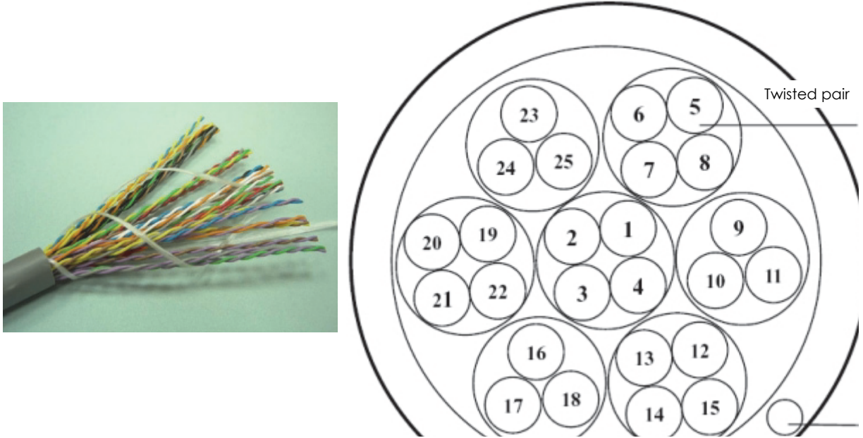
Figure 291 Telco-50 Cable Structure
