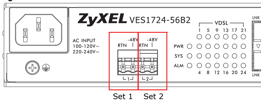
Figure 12 VES1724-55C and VES1724-56B2 DC Power Terminals
