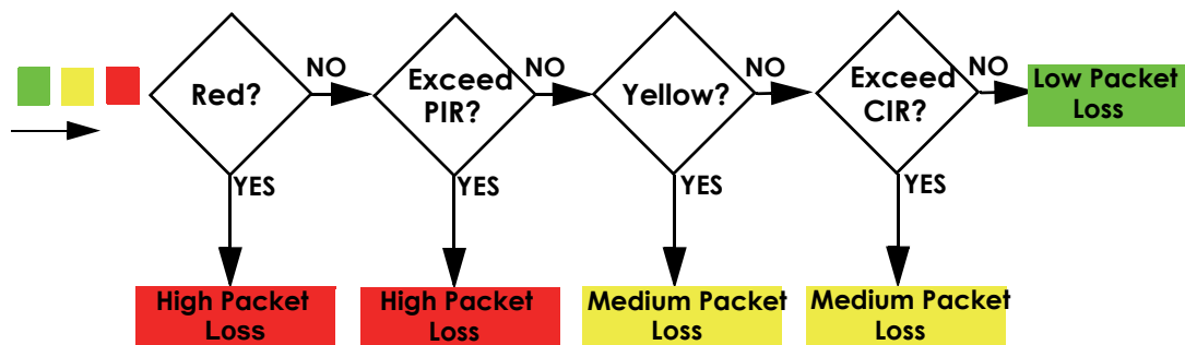
Figure 224 TRTCM-Color-aware Mode
