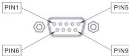
Figure 19 Alarm Port: Pin Assignment
