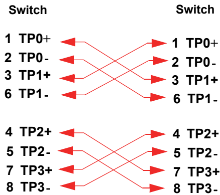
Figure 289 Twisted-Pair 1000BASE-T Ethernet Cable Schematic
