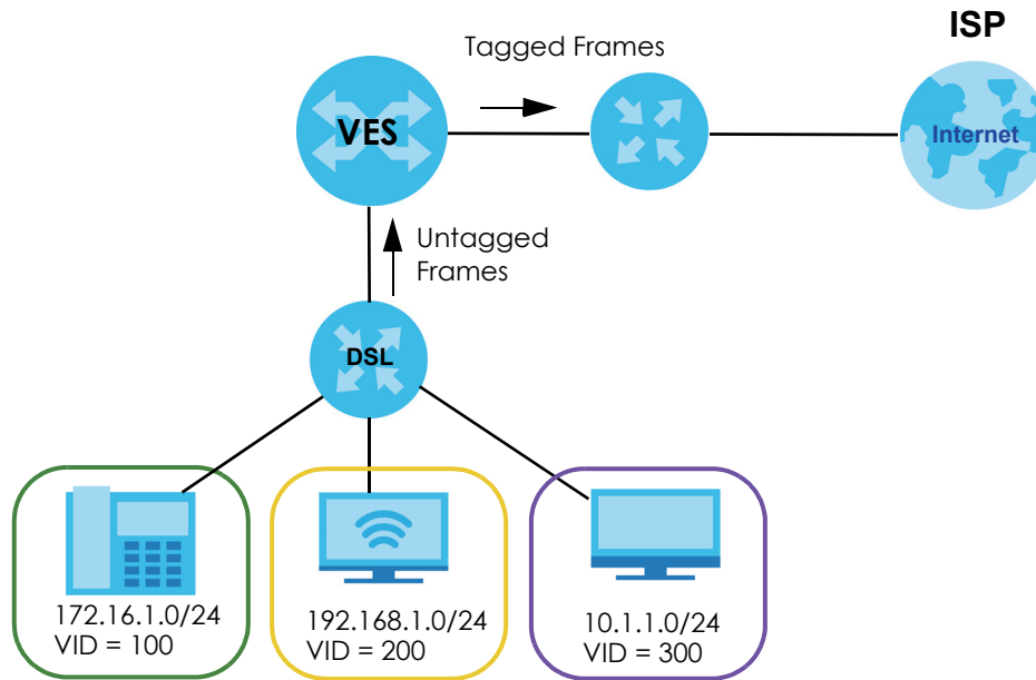
Figure 87 Subnet Based VLAN Application Example
