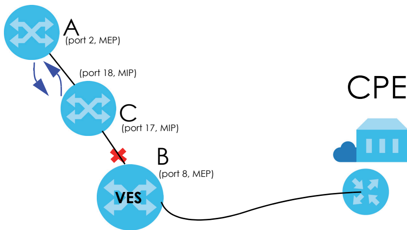
Figure 177 MIP and MEP example
