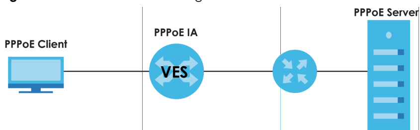
Figure 187 PPPoE Intermediate Agent Overview
