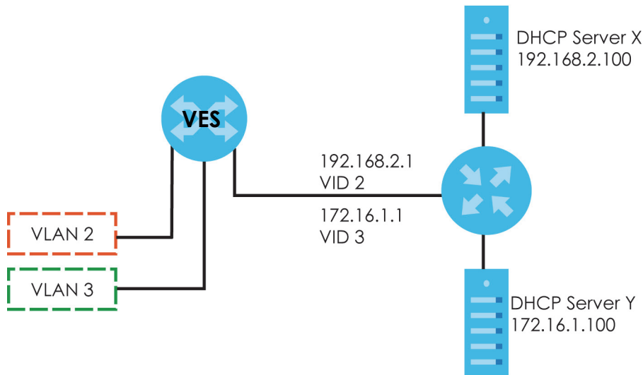
Figure 236 DHCP Relay for Two VLANs
