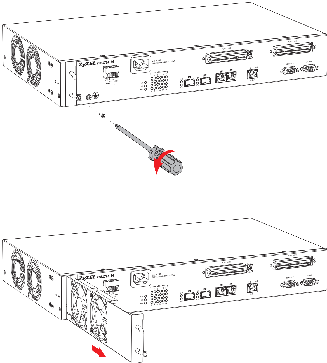
Figure 20 Removing the Fan Module
