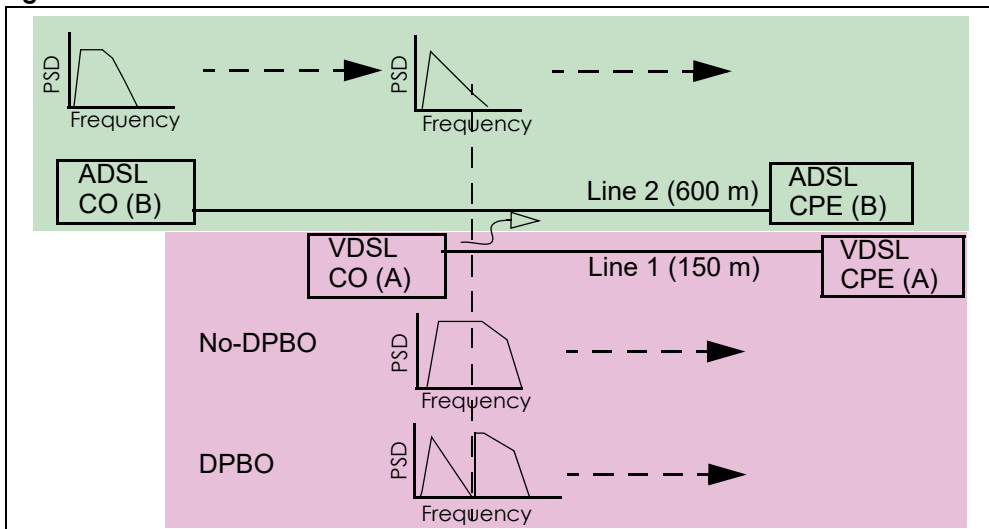
Figure 61 DPBO Resolves Downstream Far-End Crosstalk
