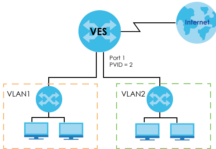
Figure 28 Initial Setup Network Example: Port VID
