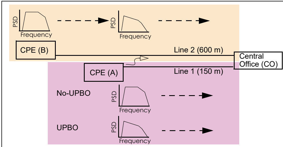
Figure 60 UPBO Resolves Upstream Far-End Crosstalk
