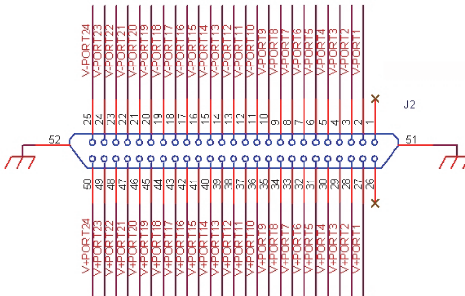
Figure 286 Hardware Telco-50 Female Pin Assignments
