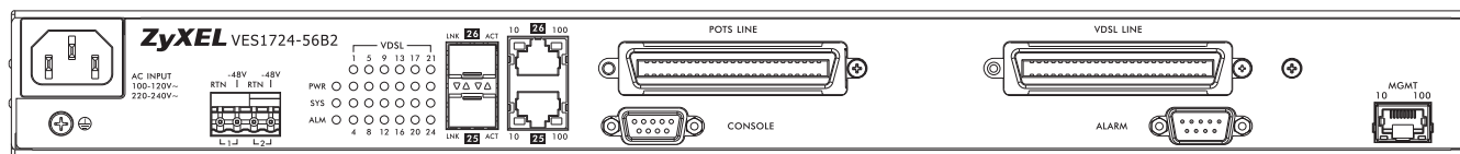
Figure 11 VES1724-56B2 Front Panel
