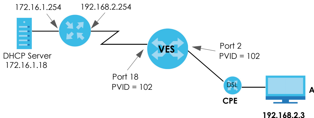
Figure 29 Tutorial: DHCP Relay Per VLAN Scenario
