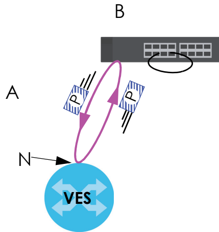
Figure 173 Loop Guard - Probe Packet
