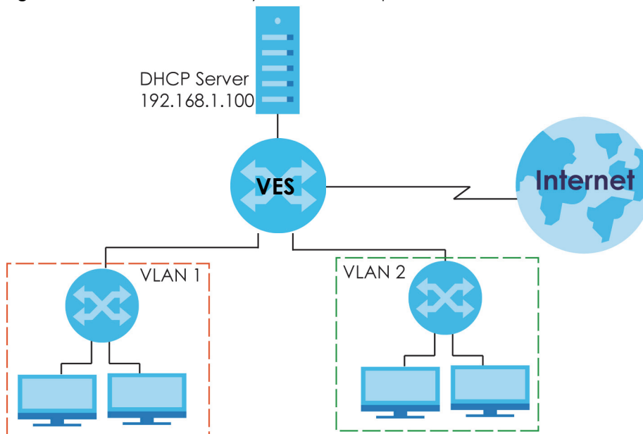
Figure 233 Global DHCP Relay Network Example
