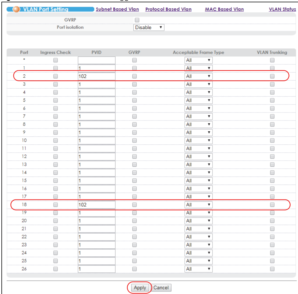
Figure 33 Tutorial: Set PVID for Untagged Frames Received on Ports 2 and 18
