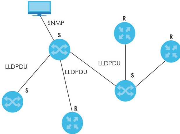
Figure 198 LLDP Overview
