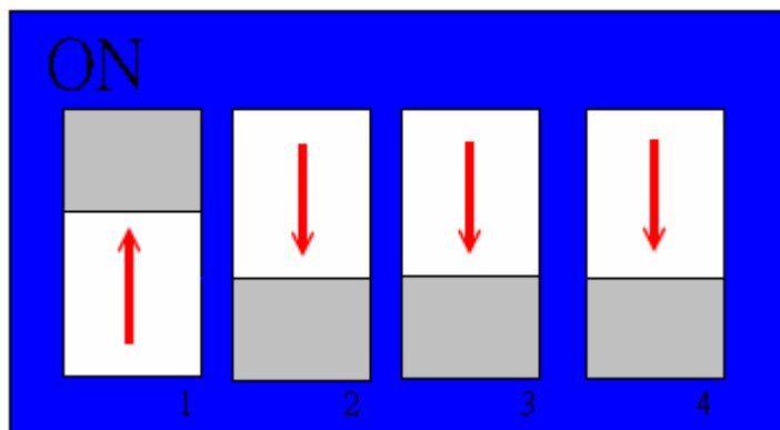
Figure 3.4 DIP switch setting
