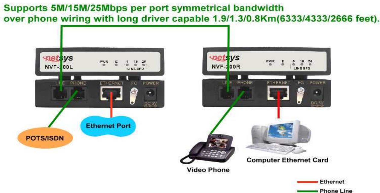
Figure 2.1 VDSL Point-to-Point application
