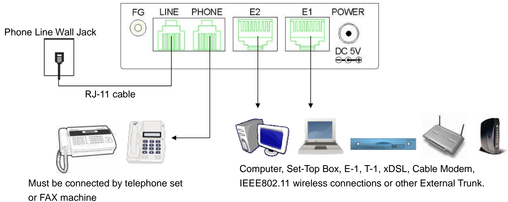
Figure 3.2 Ethernet Connecting Application Diagram
