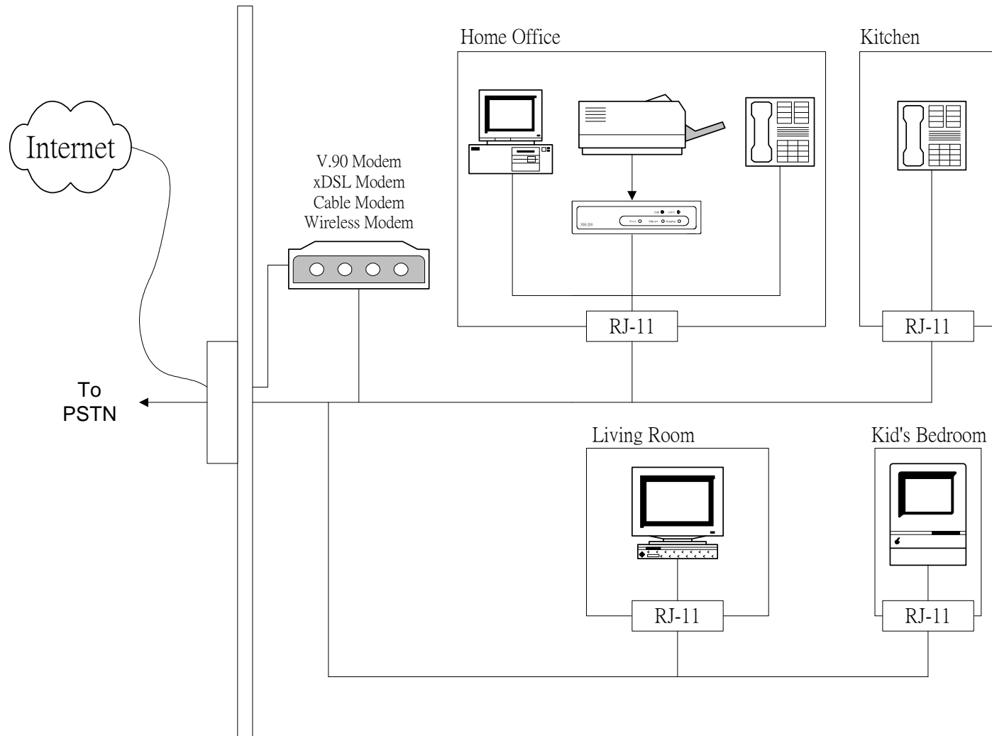
Figure 4.1 Application for home networking diagram
