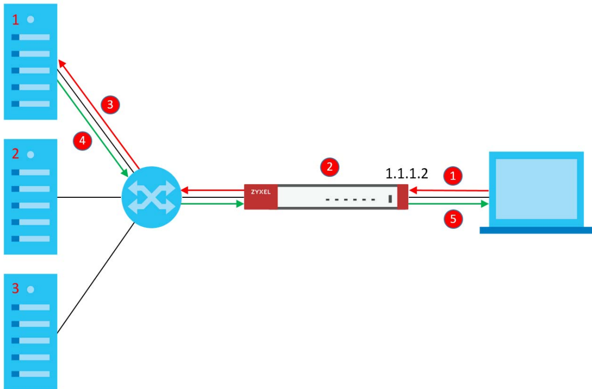
Figure 22 Load Balancing Overview
