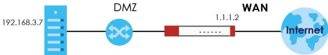
Figure 19 Public Server Example Network Topology
