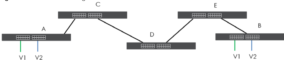
Figure 185 Port VLAN Trunking
