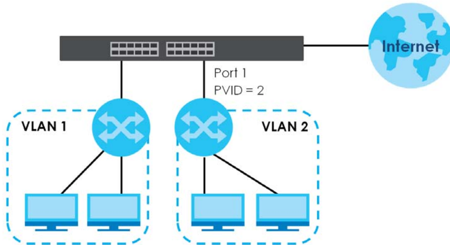
Figure 63 Initial Setup Network Example: Port VID
