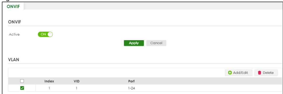
Figure 289 SWITCHING > ONVIF
