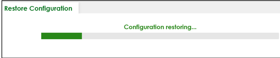
Figure 300 Configuration Restoring
