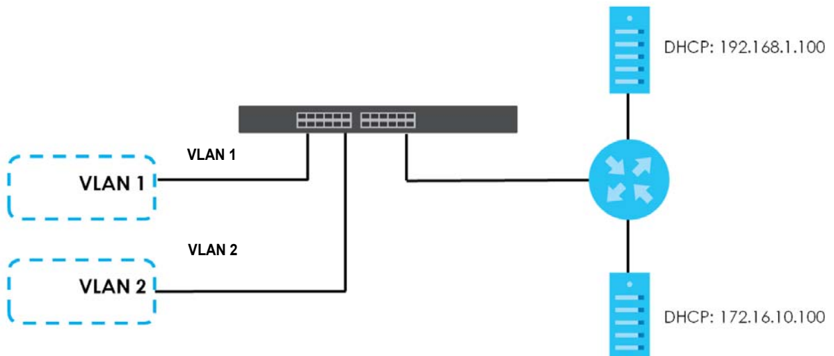
Figure 211 DHCP Relay for Two VLANs
