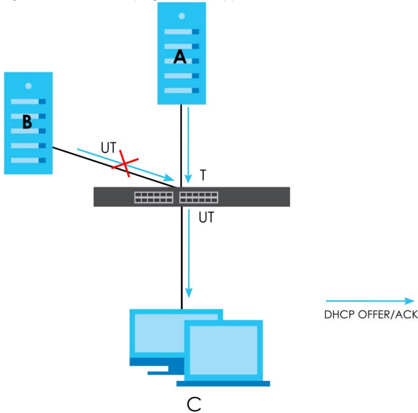
Figure 234 DHCP Snooping Example Application
