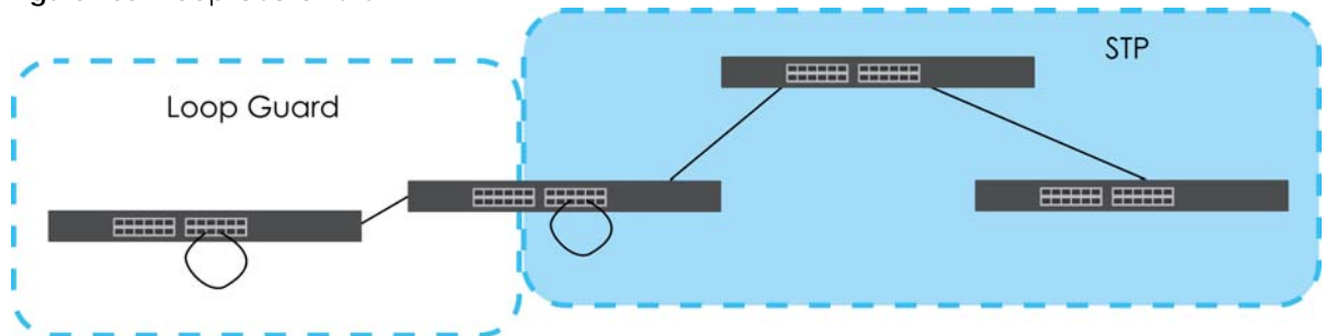
Figure 155 Loop Guard vs. STP
