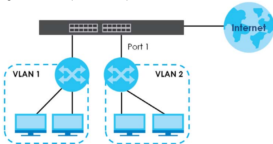
Figure 62 Initial Setup Network Example: VLAN
