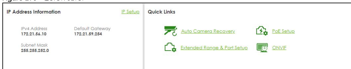
Figure 270 QUICK SETUP
