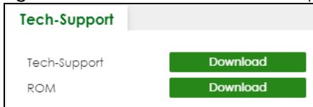
Figure 308 MAINTENANCE > Tech-Support
