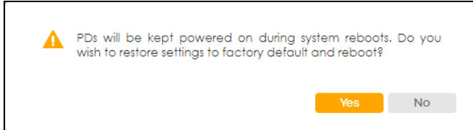
Figure 307 Reboot Confirmation
