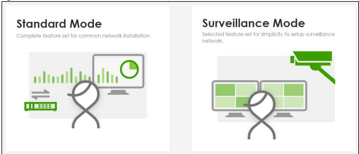
Figure 36 Select Mode
