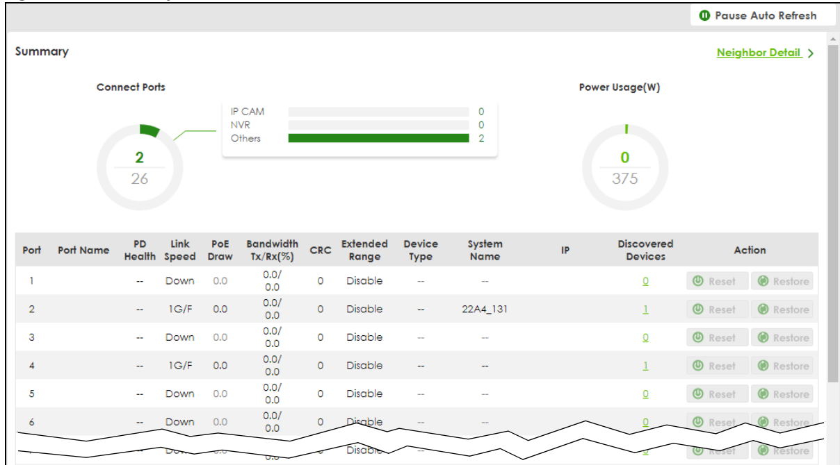
Figure 268 Summary
