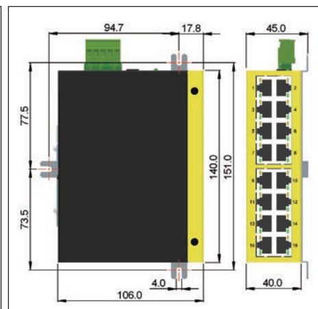
Panel Mounting Dimension
