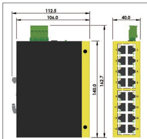
DIN-Rail Mounting Dimension
