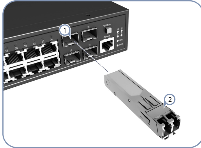
Figure 7: Inserting an SFP Transceiver into a Slot
