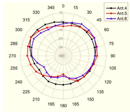
5GHz Elevation-Plane
