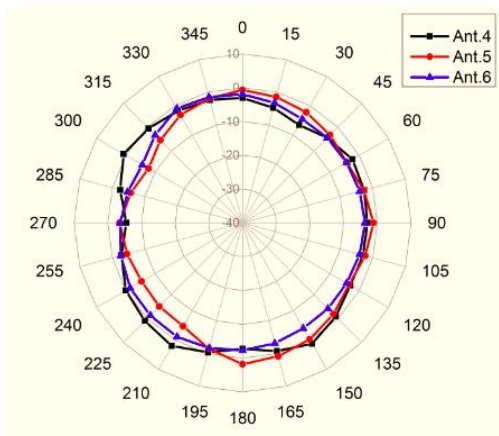
5GHz Azimuth-Plane
