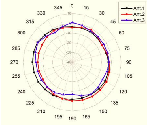
5GHz Azimuth-Plane
