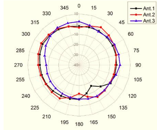
5GHz Elevation-Plane
